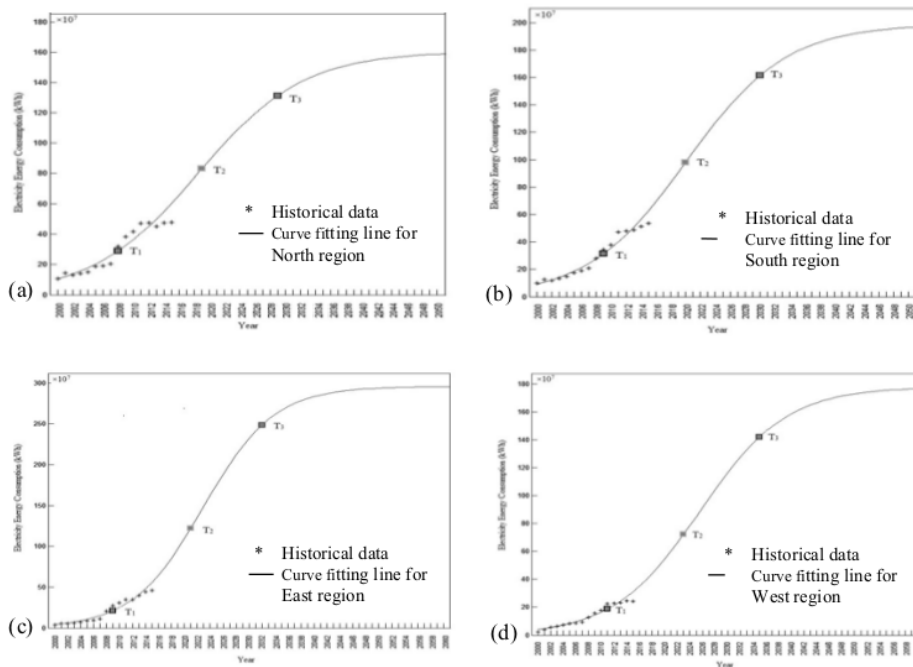
Figure 4 (a)(b)(c)(d). Logistic curve models for each service area.
