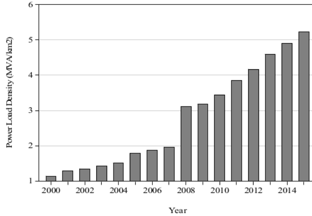
Figure 5. Power load density for Makassar.
